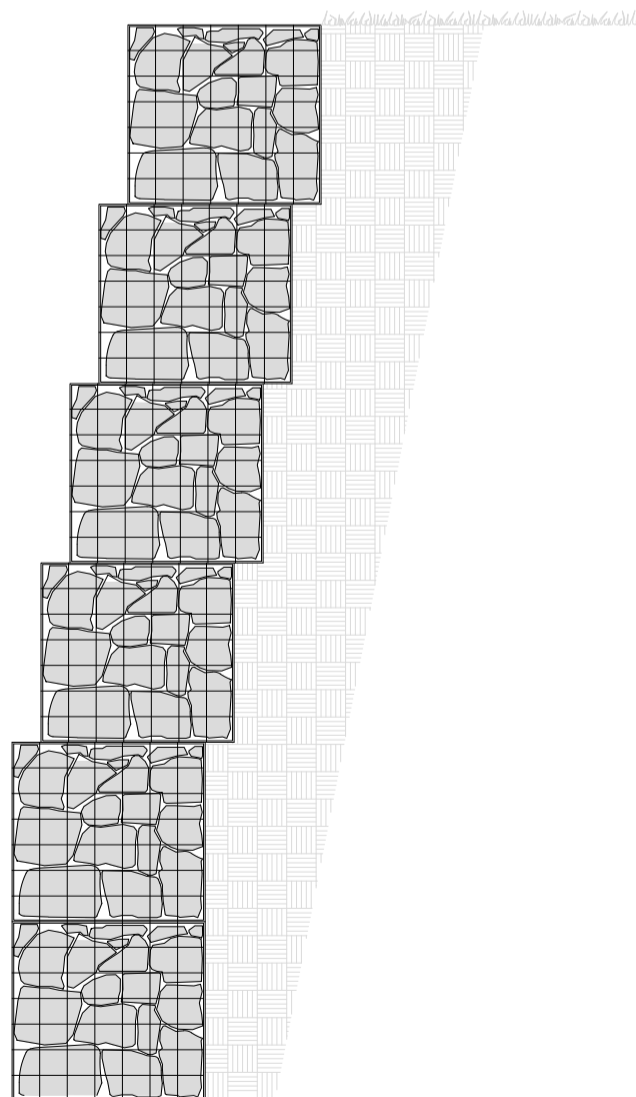
6.0m RETAINING WALL ELEVATION
