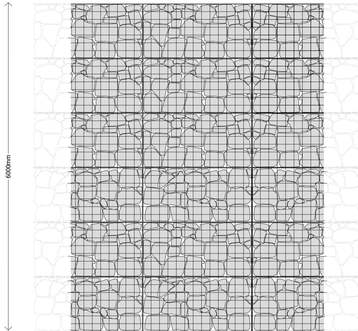
6.0m RETAINING WALL ELEVATION
